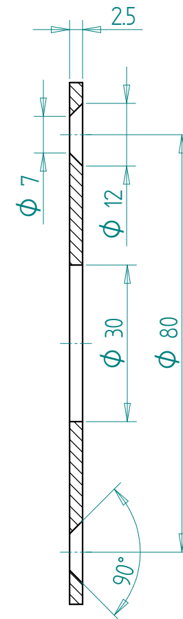
CORPO SP. 2.5mm BODY TH. 2.5mm
