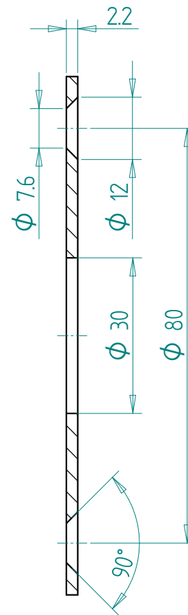
CORPO SP. 2.2mm BODY TH. 2.2mm
